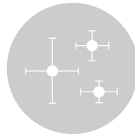
Error Bars
