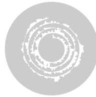
Spiral Plot
