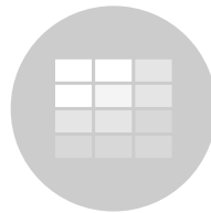
Heat Map
