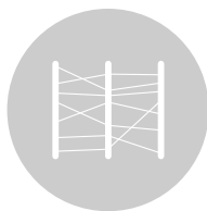
Parallel Coordinates
